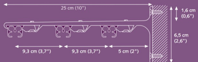
Wall bracket aluminium triple 25 cm (10'')
