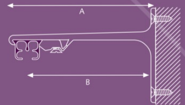
Wall bracket aluminium single A) 7,5 cm (3''), B) 6,3 cm (2,5'') A) 10 cm (4''), B) 8,8 cm (3,5'')
